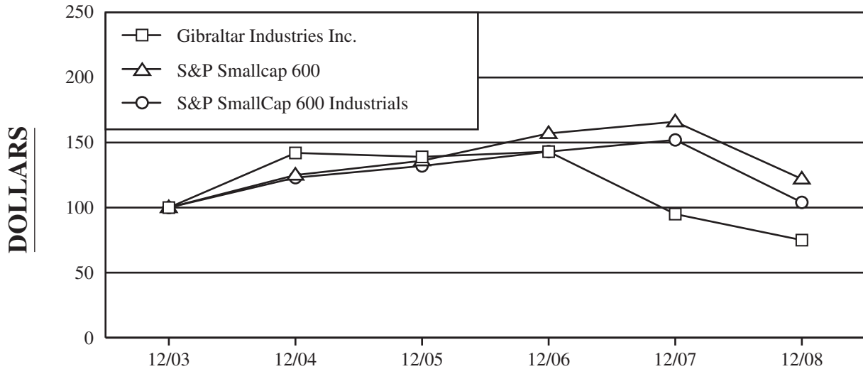
COMPARISON OF 5 YEAR CUMULATIVE TOTAL RETURN* Among Gibraltar Industries Inc., The S&P Smallcap 600 Index And The S&P SmallCap 600 Industrials
